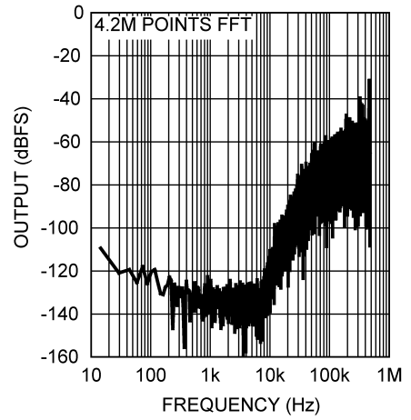
Noise vs. Frequency @ CLOCK = 960 kHz, 8 kHz Audio BW
