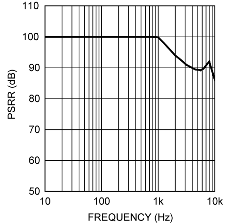
PSRR vs. Frequency @ CLOCK = 1.2 MHz
