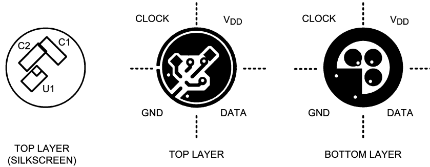
FIGURE 11. PCB Layout
